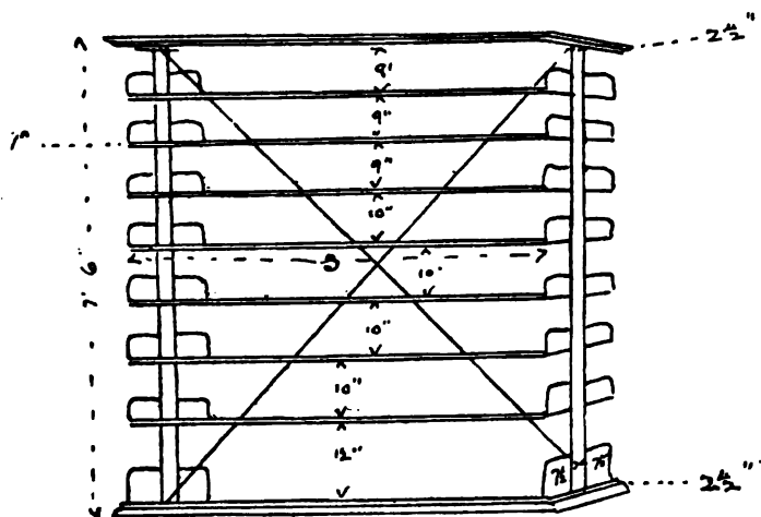
FIG. 37.—Rough Diagram of Standard Iron Bookcase, 7 feet 6 inches \times 3 feet 2 inches \times 15 inches.
